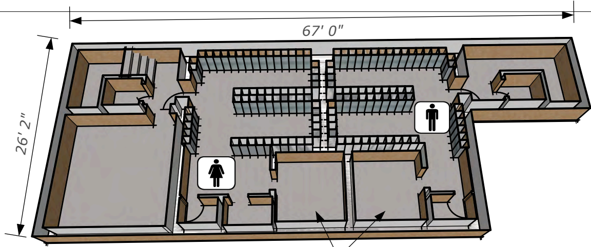
LOCKER ROOMS FLOOR PLAN
